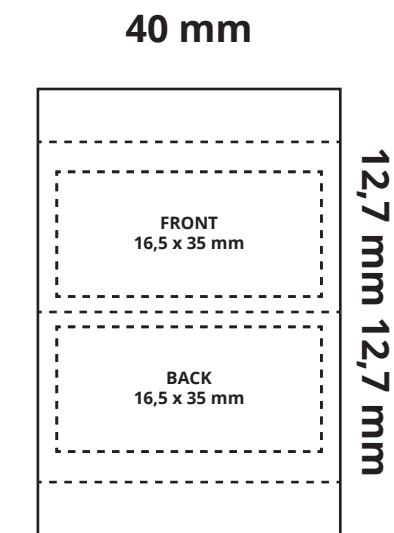
LABEL 40 x 15 mm (folded)
